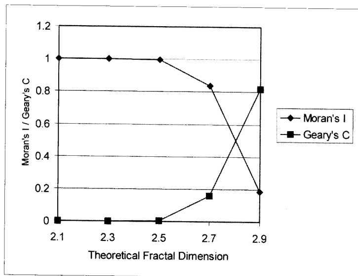
Figure 4. Relationship between theoretical fractal dimension and spatial autocorrelation indices.
