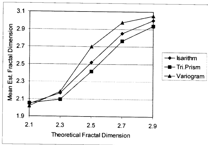
Figure 3. Comparison between mean estimated fractal dimension and theoretical fractal dimension.
