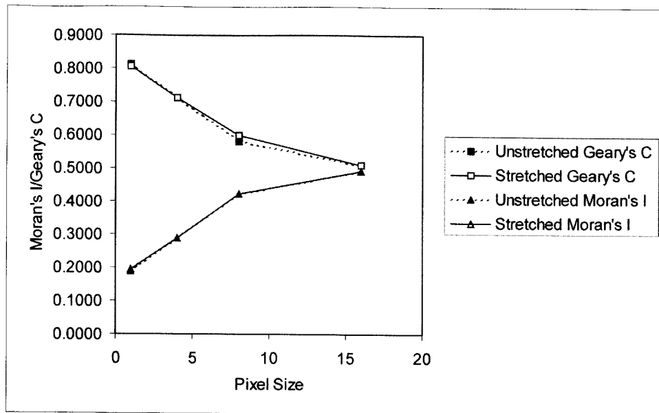
Figure 6. Effect of resampling and contrast stretching on Moran's I and Geary's C.
