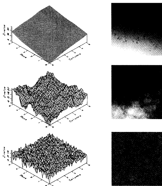
Figure 1. Three simulated surfaces and corresponding images from top to bottom, D = 2.1, 2.5 , and 2.9 .
