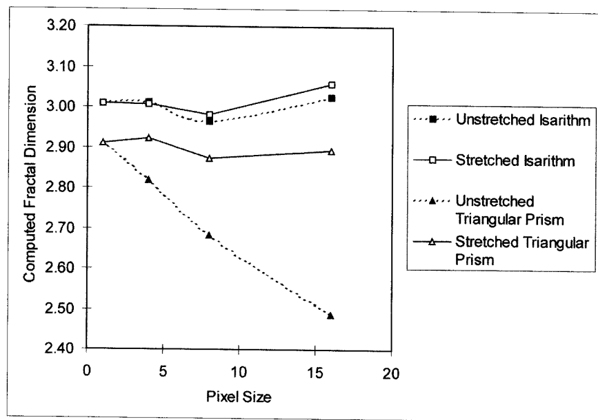
Figure 5. Effect of resampling and contrast stretching on computed fractal dimensions.
